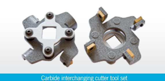
Carbide interchanging cutter tool set
